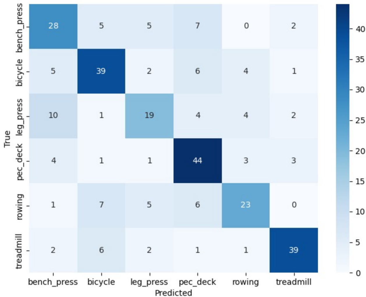
Confusion Matrix
