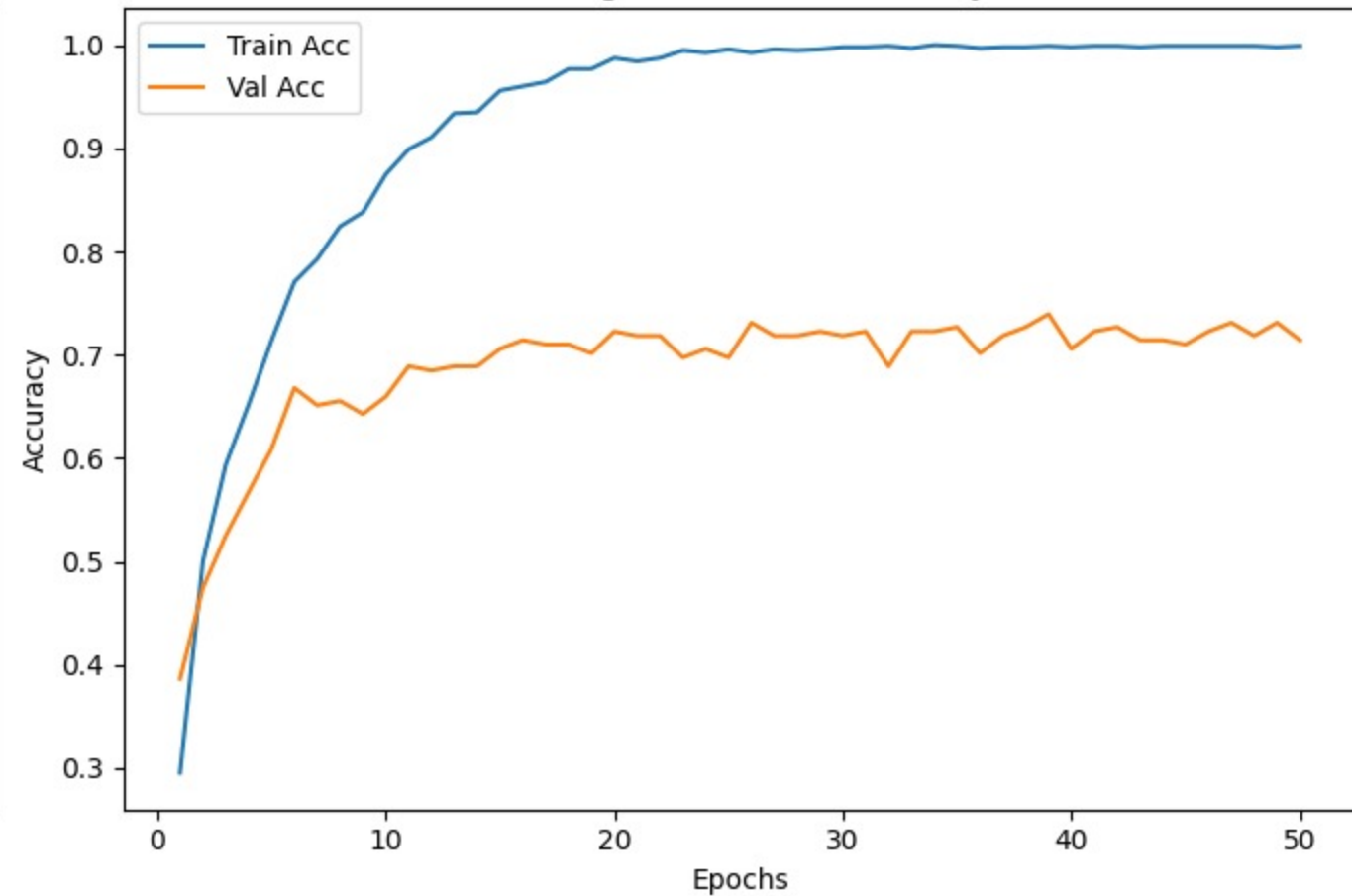
Training &amp; Validation Accuracy
