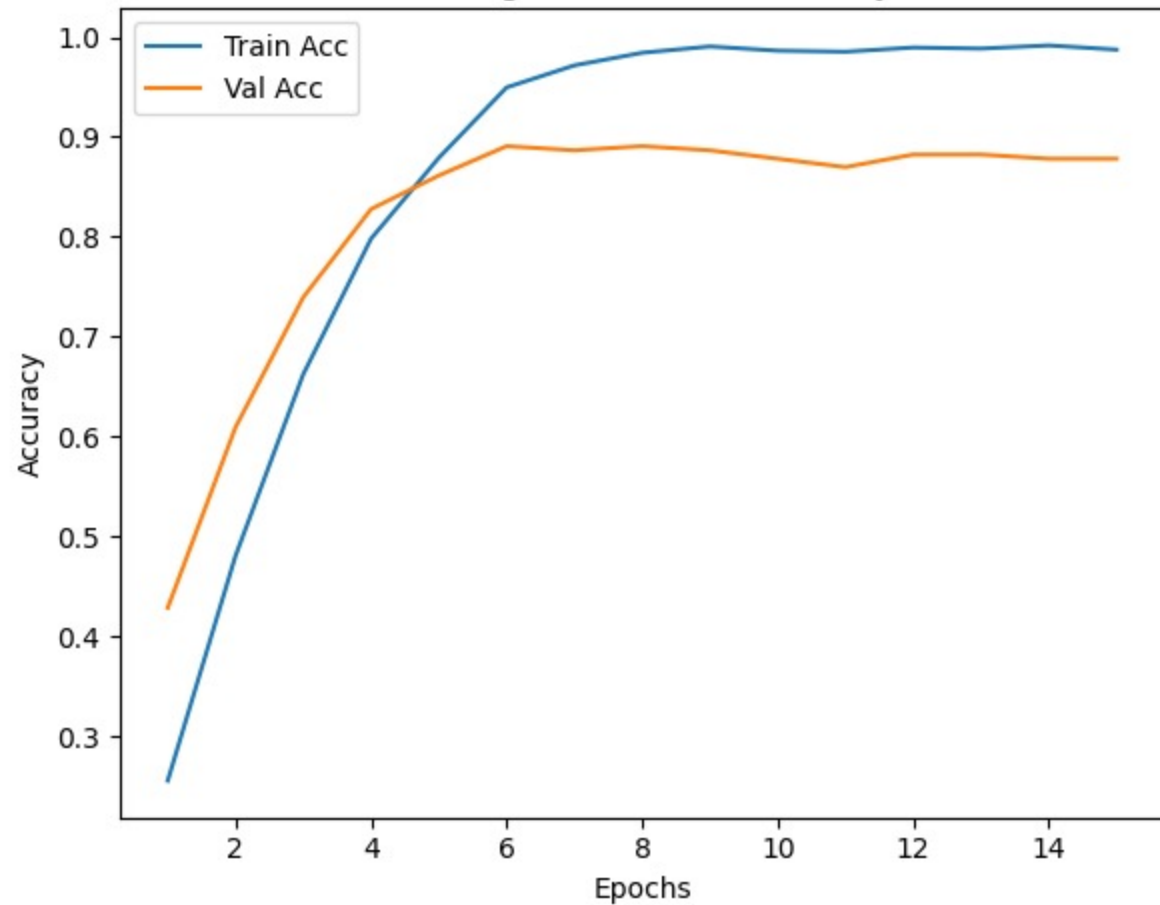
Training &amp; Validation Accuracy
